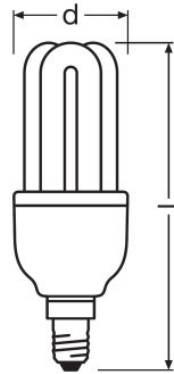
D STICK 8 W/827 220...240 V E14, D STICK 8 W/840 220...240 V E14, D STICK 8 W/865 220...240 V E14
